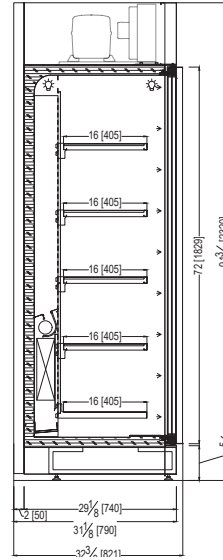
OPTIONAL: TOP MOUNTED CONDENSING UNIT
