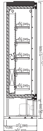
OPTIONAL: SLIDING DOORS ONLY IN SOLID SIDES AND 2100, 2800 MODELS
